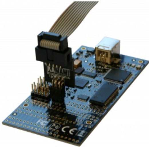
KAmoISP and AVR Dragon
